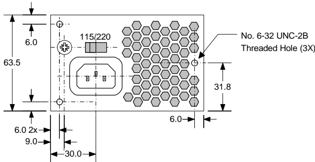
Figure 2 Mechanical Outline
