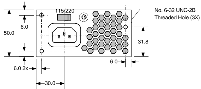
Figure 5 50mm Profile Mechanical Outline
