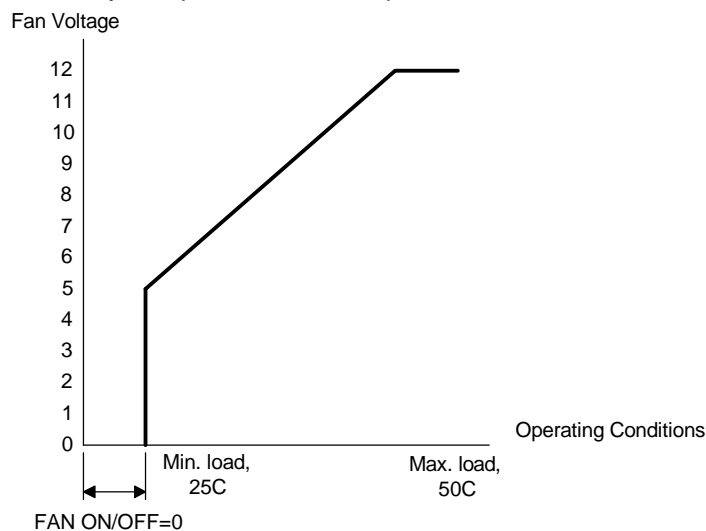
Figure 3 Fan Speed
