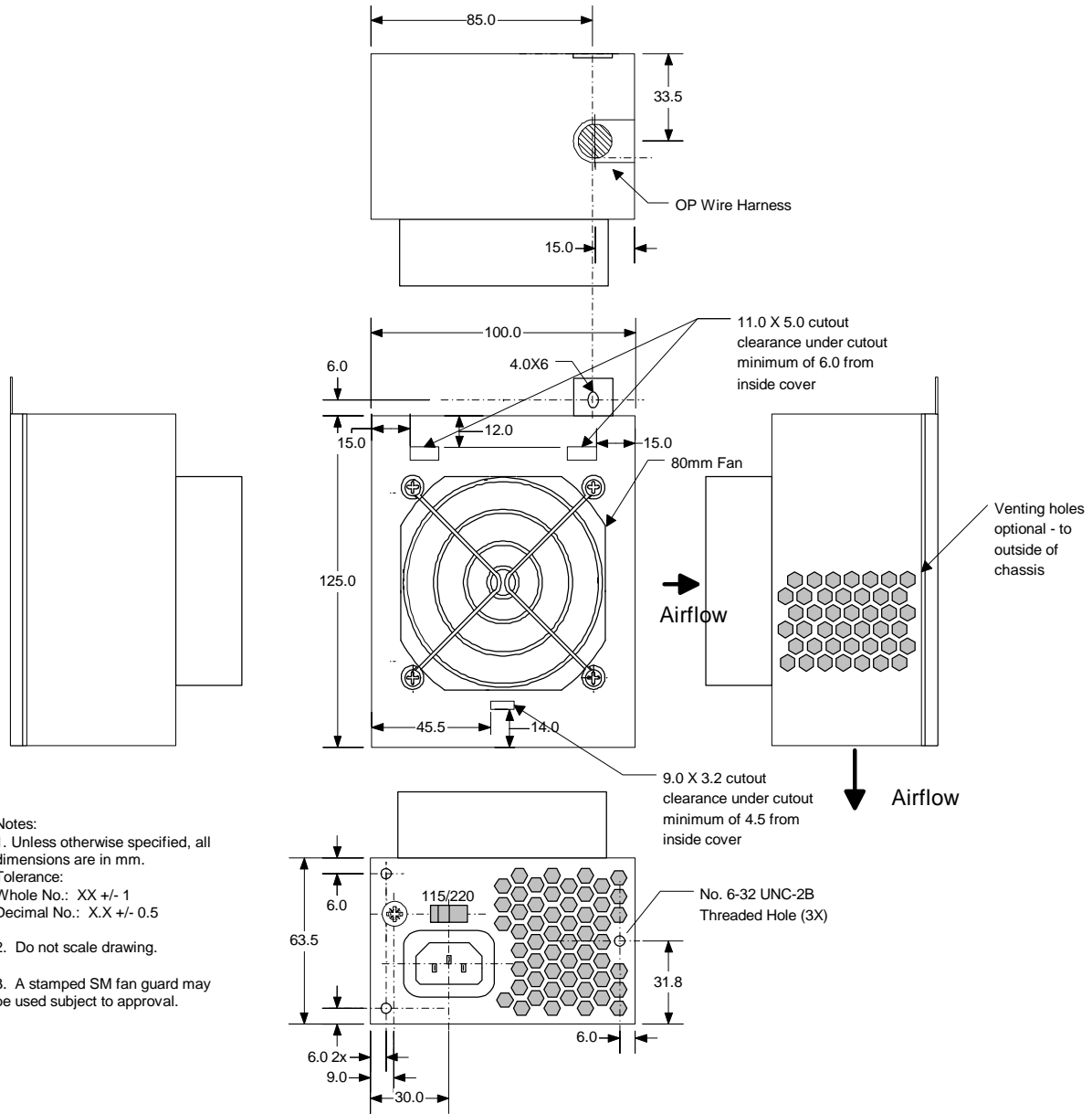
Figure 6 Top Mount Fan Profile Mechanical Outline
