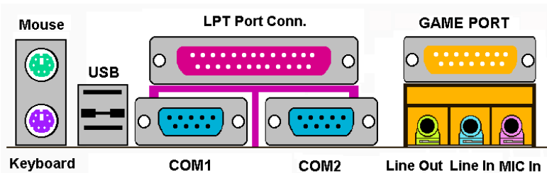
Figure 2-13. VL6 back panel connectors
