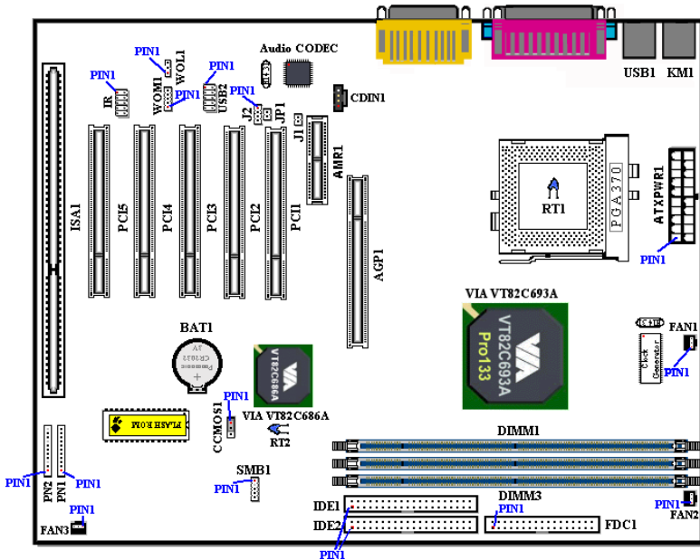
Figure 2-7. All Connectors and Headers for the VL6
