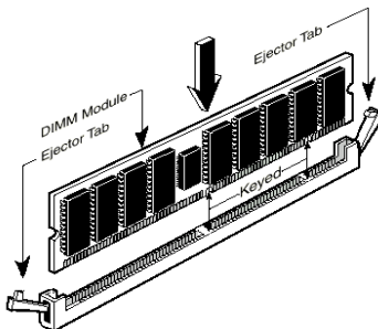
Figure 2-6. Memory module installation
