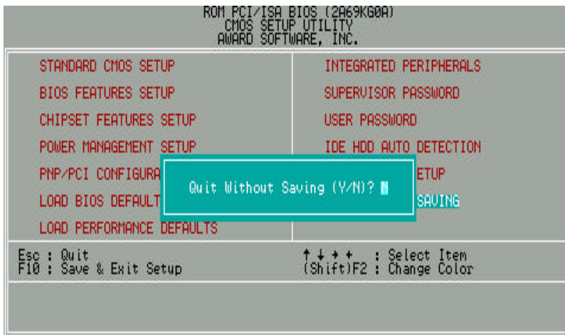
Figure 4.13: Exit Without Saving
