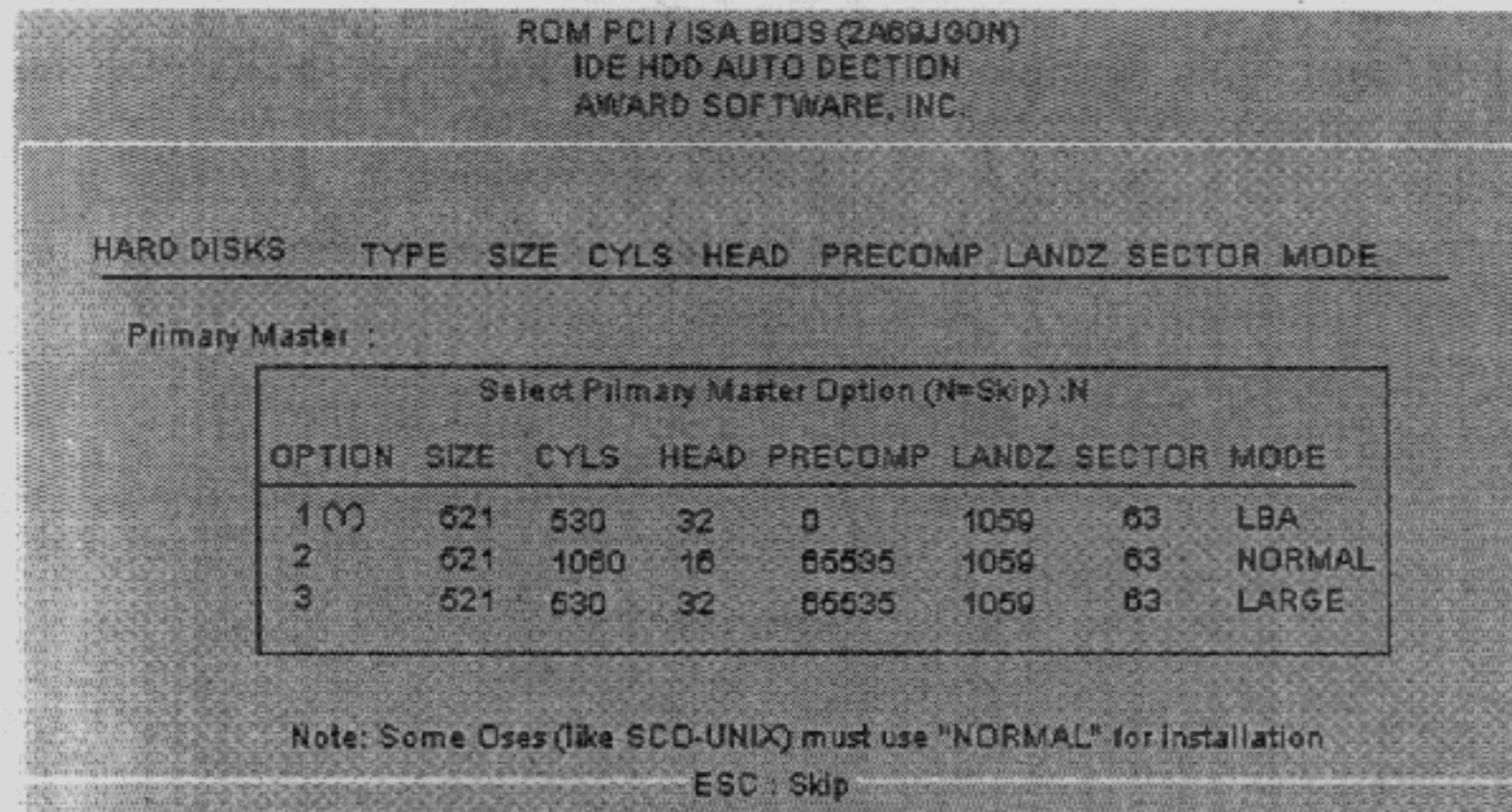
Figure 4.11: IDE HDD Auto Detection
